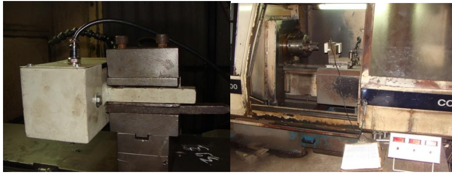
Figure 3 Experimental set up
