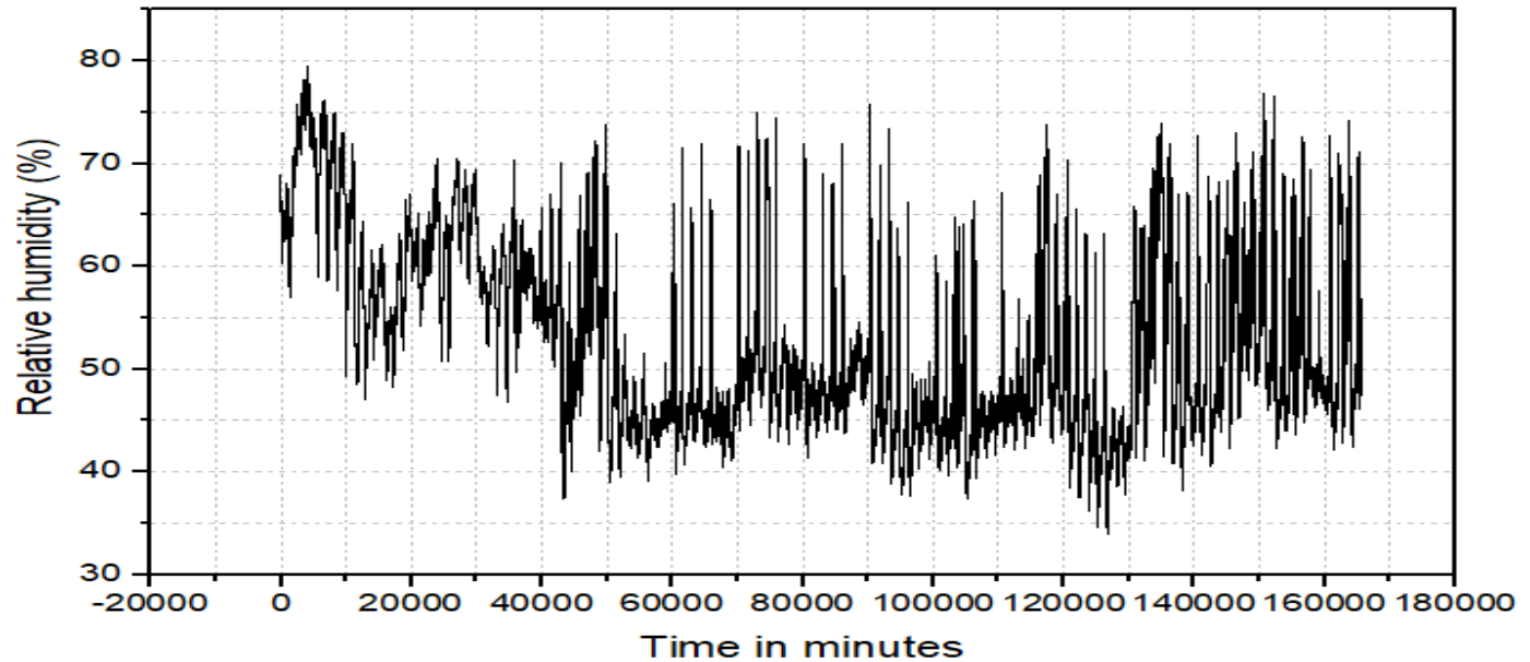
Relative humidity monitoring per minute during the period from 06 November 2018 to 28 February 2019
