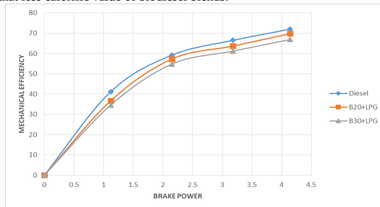
Figure 10: Brakepower vs Mechanical efficiency
