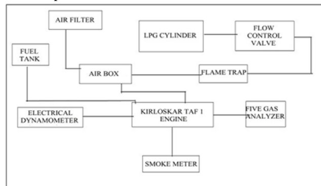
Figure 3: Experimental layout
