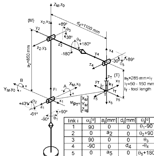
Fig.2. D-H link coordinate frames and kinematic parameters
