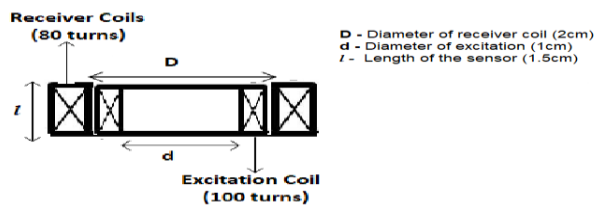
Figure 2.1 The excitation-receiver sensor.
