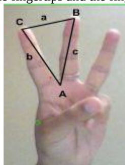
Figure 2. Finding convexity defect Convexity defects obtained, is a structure that returns four values, start point, end point, farthest point and approximate distance to farthest point, out of which three have been used.
