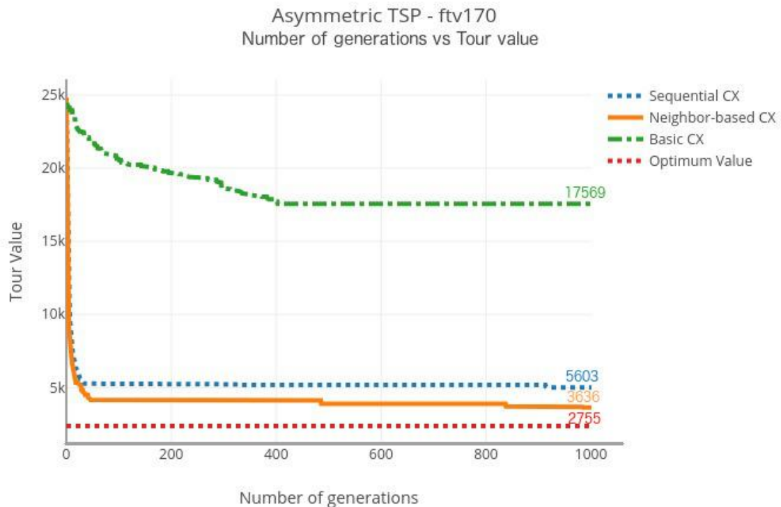
Figure 2. Performance of different crossover operators on Asymmetric TSP instance fvtv70(71 nodes) [2]
