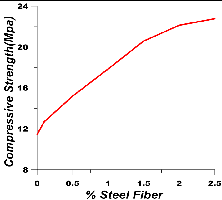
Fig. 8 Compressive Strength Test
