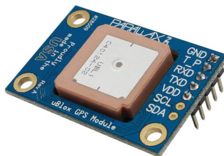
Figure 3.1.2: GPS Module
