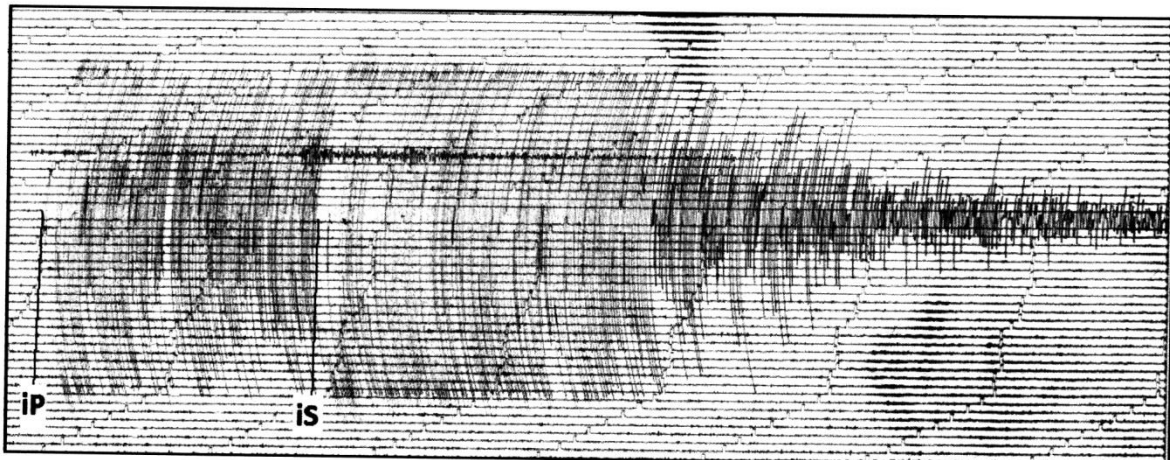
Fig. 1: Earthquake showing impulsive phases
