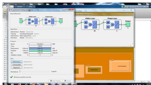
Fig7: Train Network
