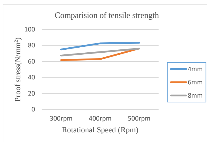
Figure 6. Comparison of tensile strength of Al-5% Si alloy with zirconia
