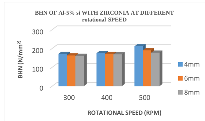
Figure5.Comparison of BHN, for different cast thickness at different speed.
