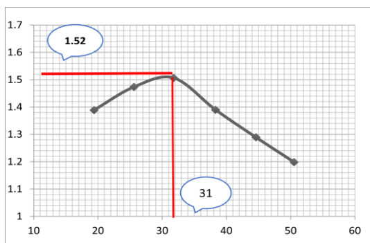
Fig 7Relation between DD and MC (Soil+3%CW)
